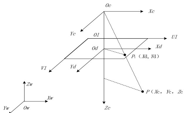
Figure 1. Camera coordinate relation
